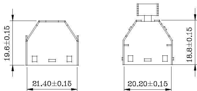
HPD-PSMBK-020-LF LEADFREE RoHS Compliant
