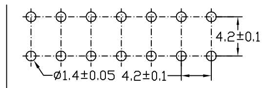
P.C.B. RECOMMENDED LAYOUT
